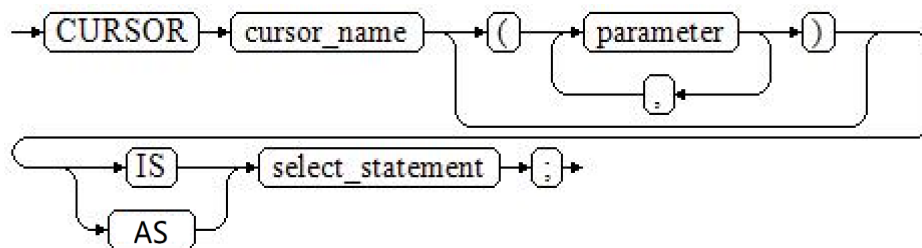
图 10-25 static_cursor_define::=
