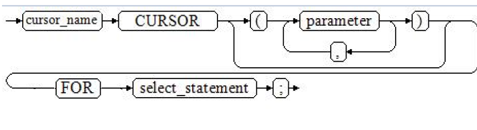
图 10-26 static_cursor_define::=
