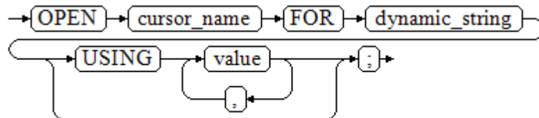
图 10-7 open_for::=
