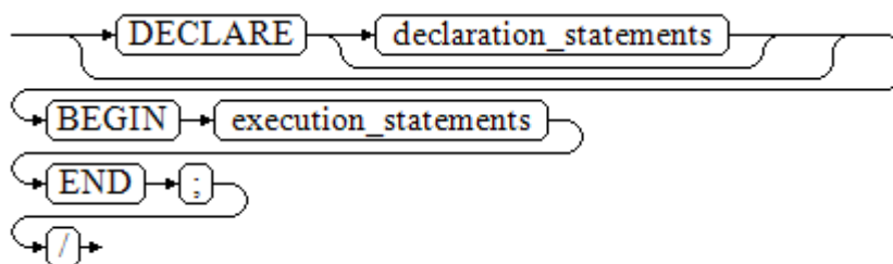
图 10-1 anonymous_block::=
